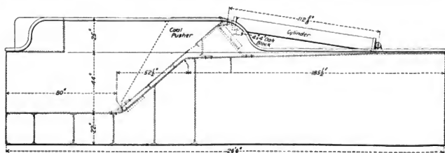
Figs. 4225-4226. Pneumatic Coal Pusher for Large Tenders. Atchison, Topeka & Santa Fe.
